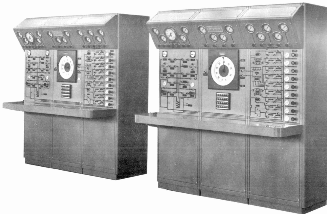
REMOTE CONTROL CONSOLES DESIGNED AND BUILT BY CRYOVAC FOR OPERATING AND MONITORING A COMPLETE CRYOGENIC SYSTEM.
